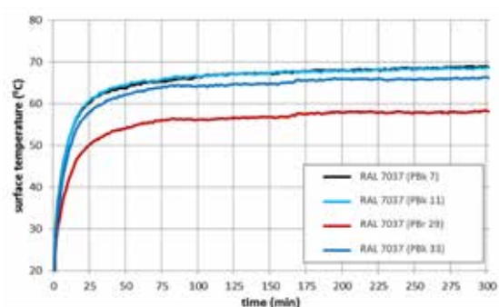
Figure 3: Heat build-up profiles of shade RAL 7037 made with different black pigments.
